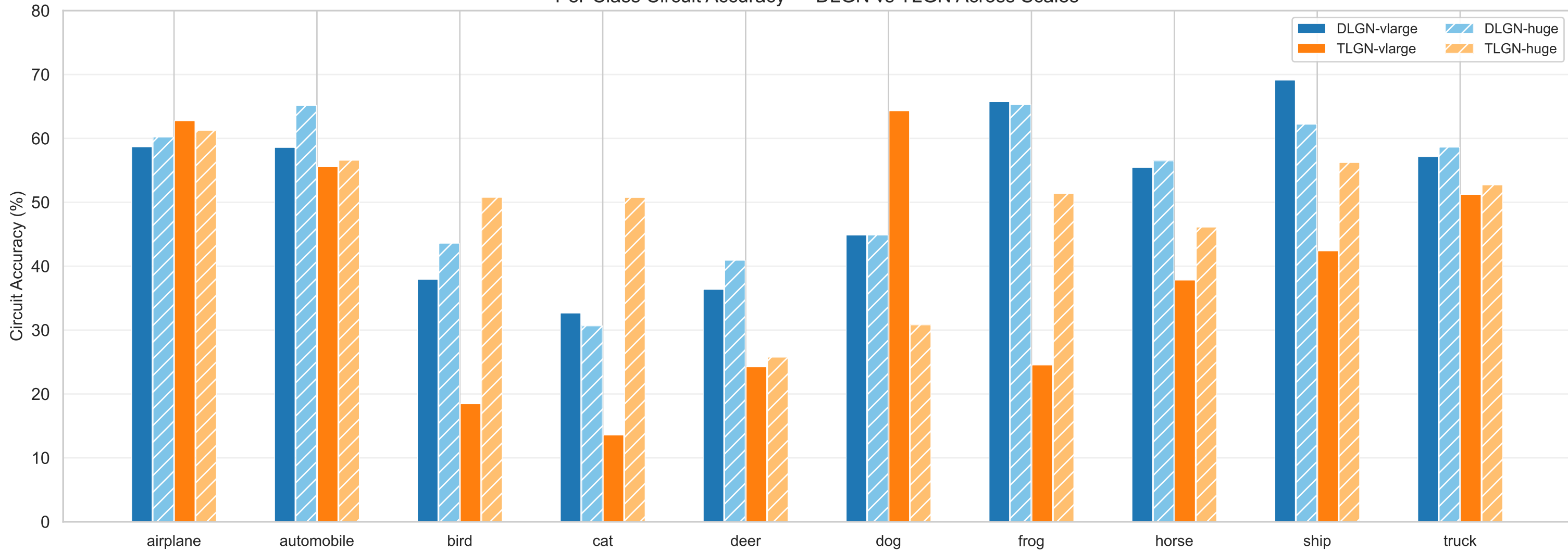
Per-Class Circuit Accuracy — DLGN vs TLGN Across Scales
