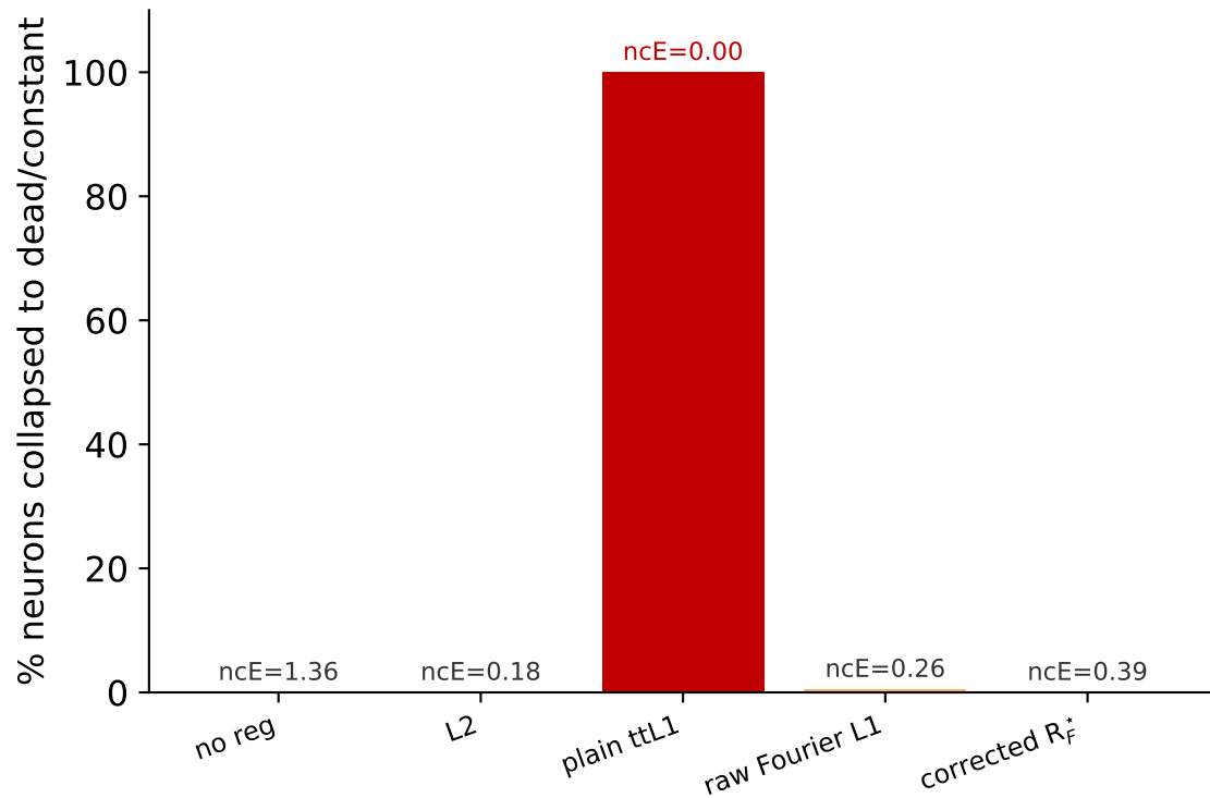
Collapse-immunity at high \beta plain ttL1 \rightarrow 100% dead; corrected R_F^* holds (floor)
