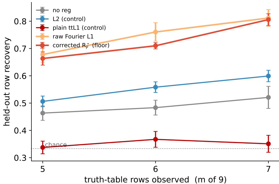
Fourier sparsity recovers gates from few rows (and it is SPECIFICALLY spectral: plain ttL1 harms)
