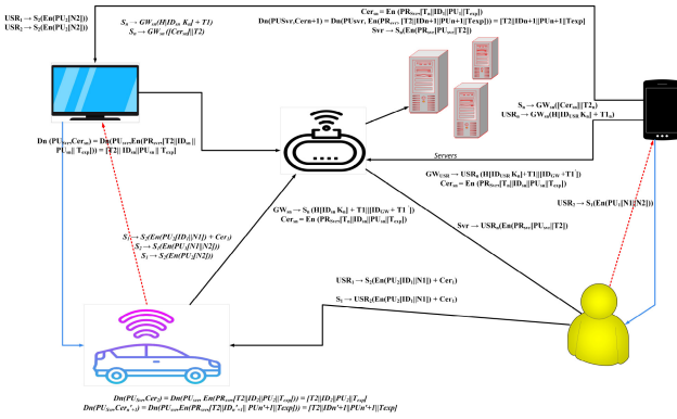
Fig. 3. LMA process between two Devices, Gateway and Server.
