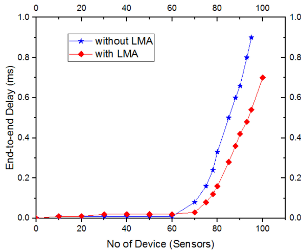
Fig. 6. End to End Delay in ms in LMA compared without LMA.
