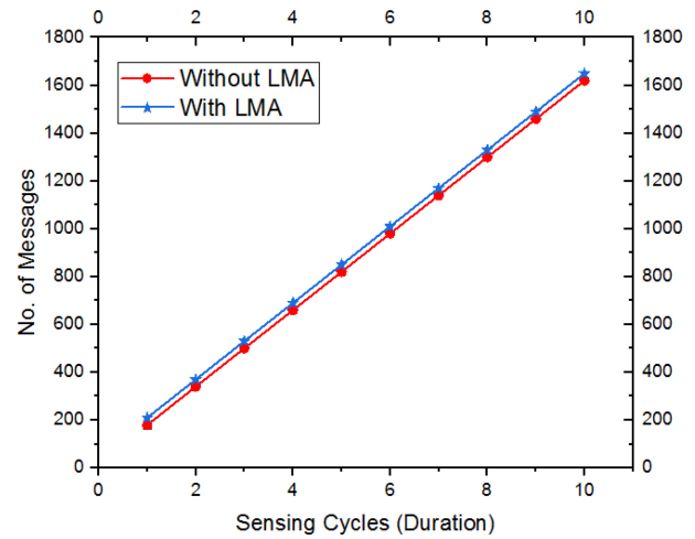
Fig. 7. No. of Messages in each Sensing Cycle.
