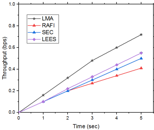
Fig. 11. LMA Throughput comparison with Other Schemes.
