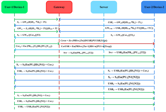
Fig. 2. LMA Sequential Flow of Messages between Users, devices, gateway and server.
