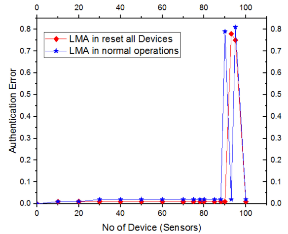
Fig. 5. Authentication Error in 100 Device in IoT network.
