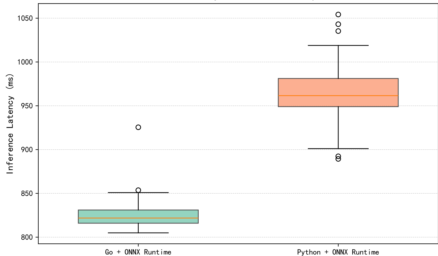
Inference Latency Distribution Comparison
