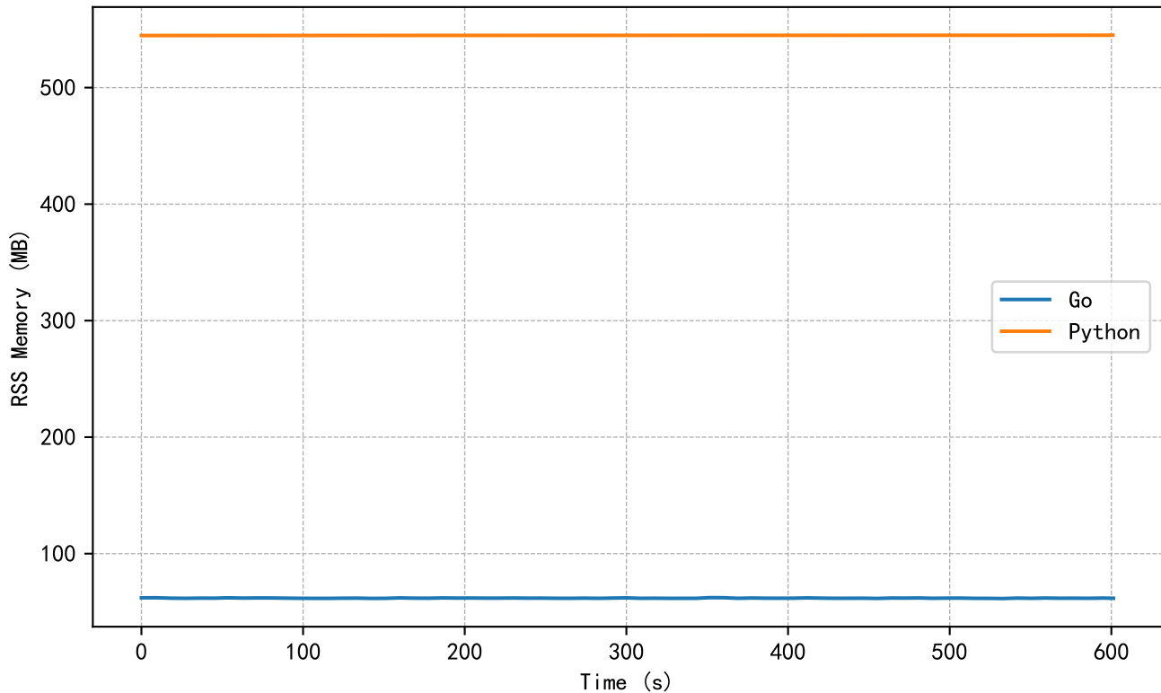
RSS Memory Usage During Long-Term Inference
