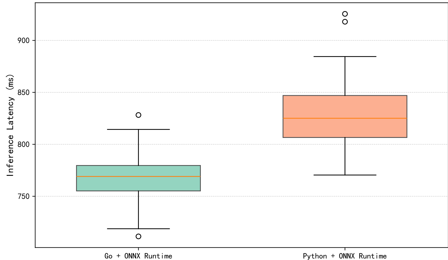
Inference Latency Distribution Comparison
