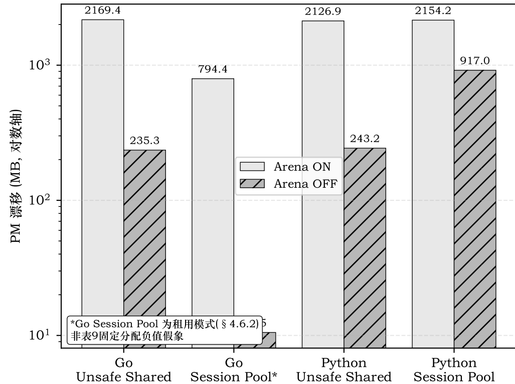
(a) Arena ON/OFF 漂移对比
