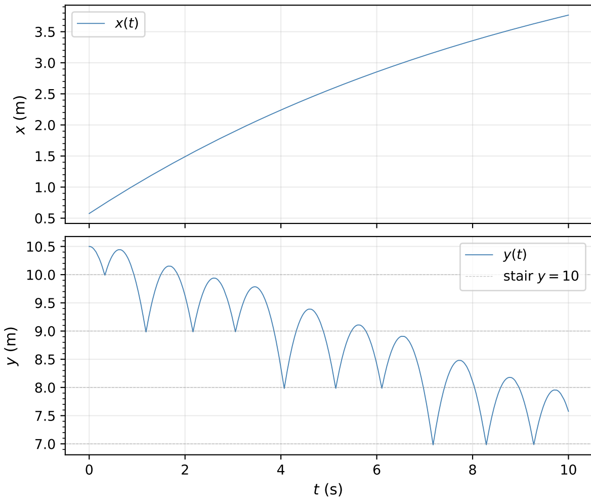
K04 §4.2 — QSS1 Bouncing Ball Downstairs ( t \in [0, 10] s)
