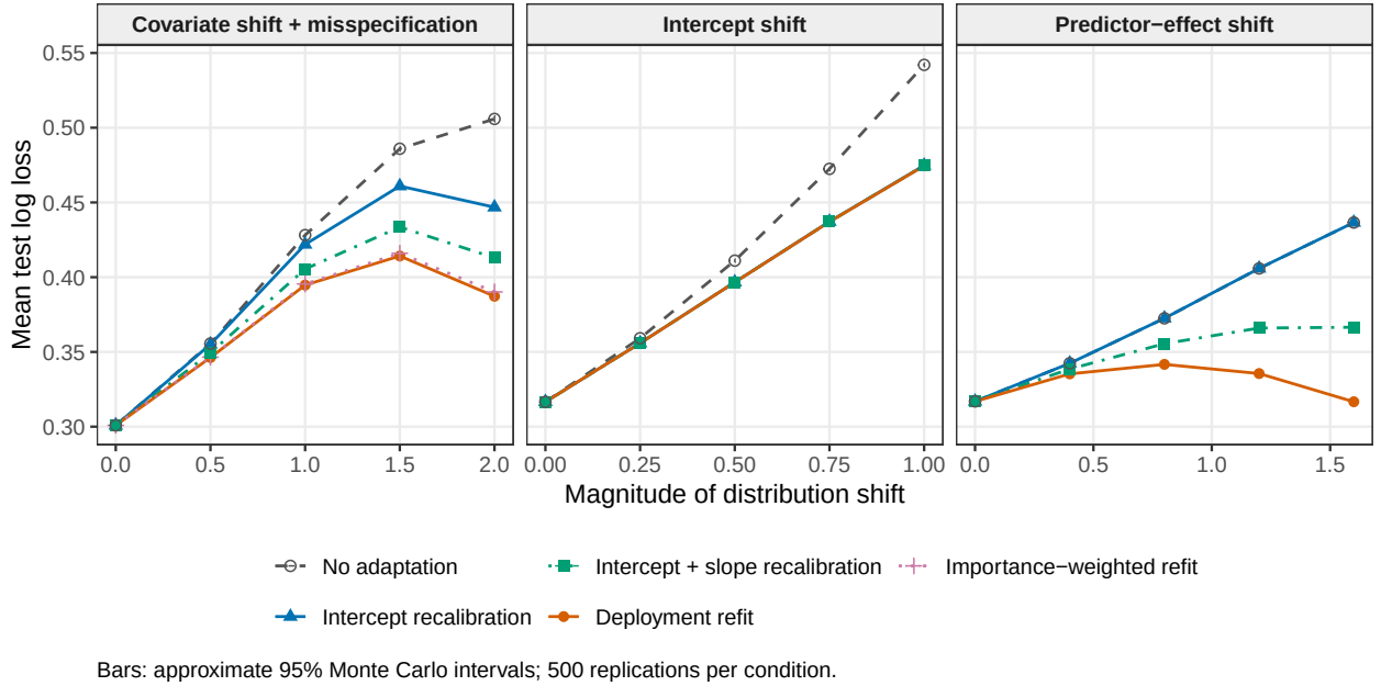
Figure 1: Probability performance after distribution shift. Lower log loss indicates more accurate probabilistic predictions.
