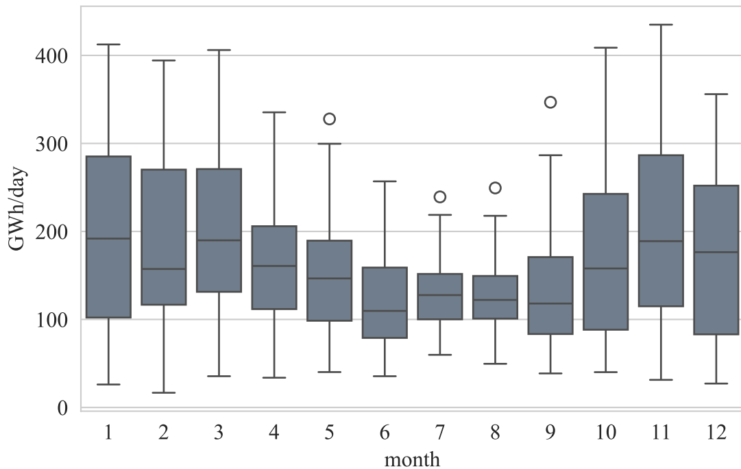
Monthly Distribution of Wind Generation
