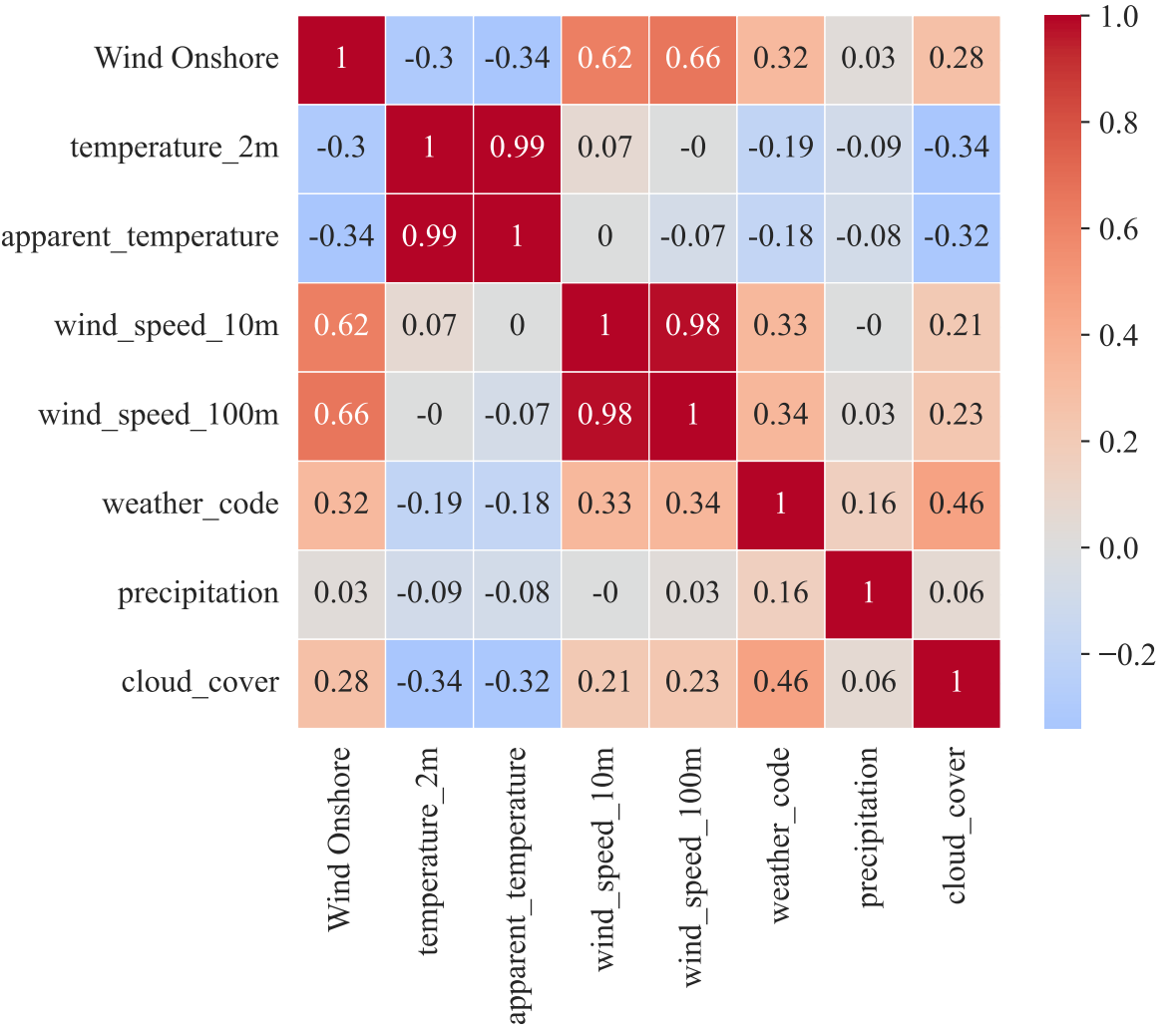
Correlation: Daily Wind Onshore Generation and Weather Features
