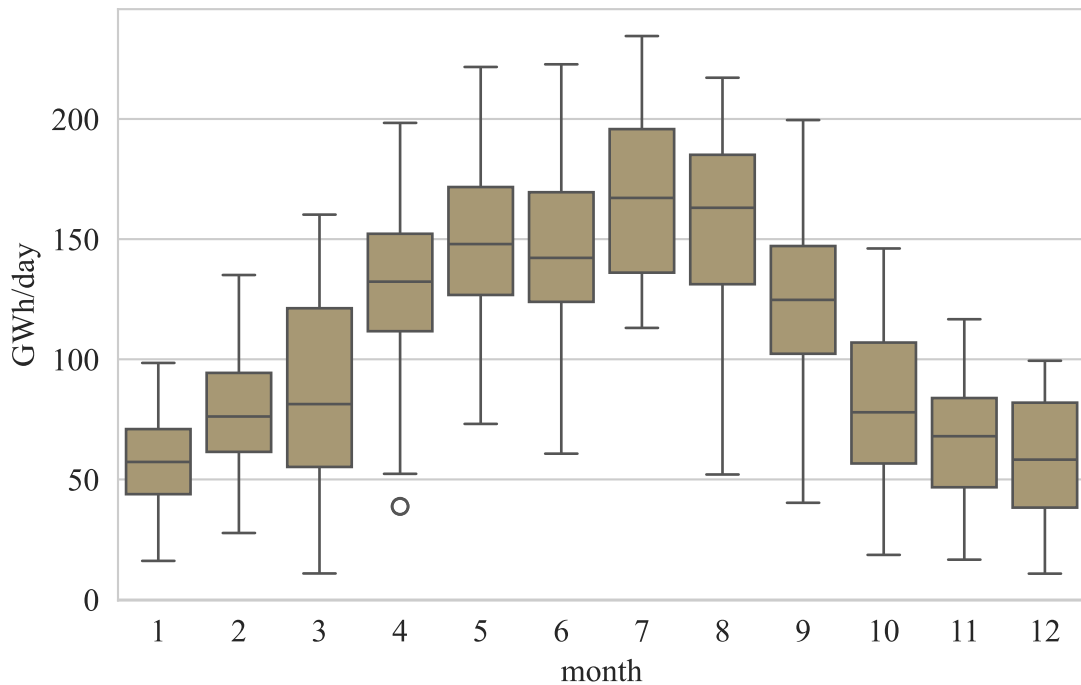
Monthly Distribution of Solar Generation
