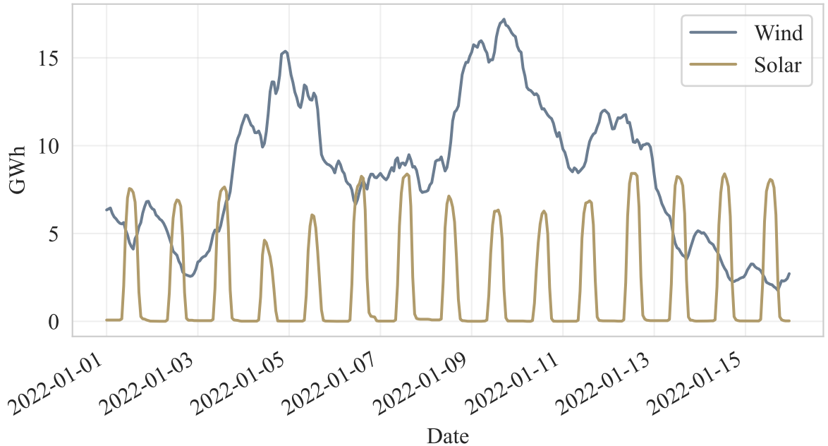
Hourly Wind & Solar Generation (First 15 days)
