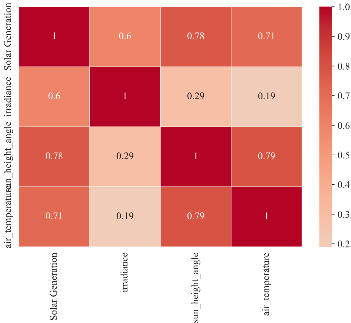
Correlation: Daily Solar Generation and Weather Features
