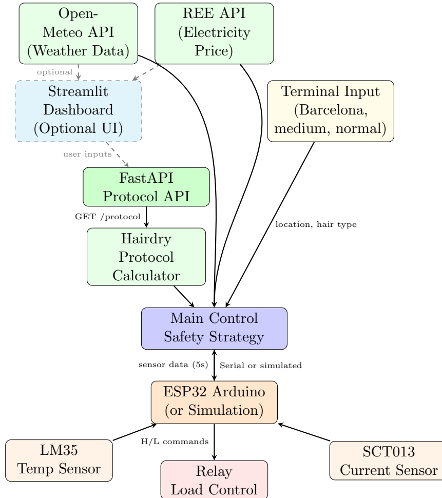
Figure 10: Software schematic.
