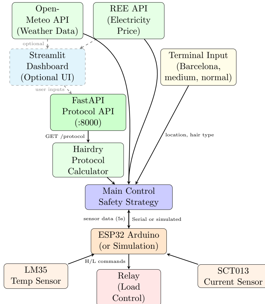
Figure 10: Software schematic showing dual operation modes: standalone terminal-based control (solid lines) with direct API access and default values, or optional dashboard interface (dashed lines). Simulation mode enables hardware-free software testing.
