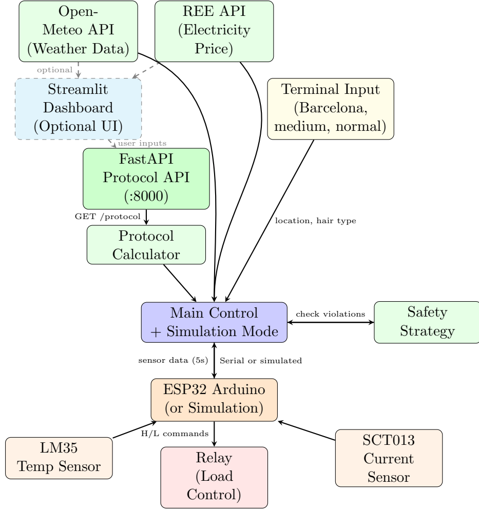
Figure 9: Software schematic showing dual operation modes: standalone terminal-based control (solid lines) with direct API access and default values, or optional dashboard interface (dashed lines). Simulation mode enables hardware-free software testing.
