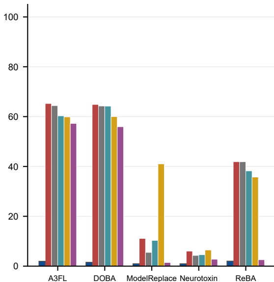
CIFAR-100
