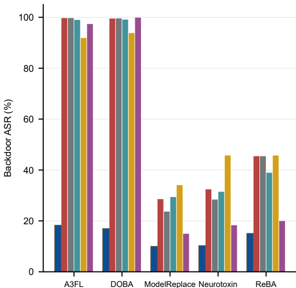
CIFAR-10
