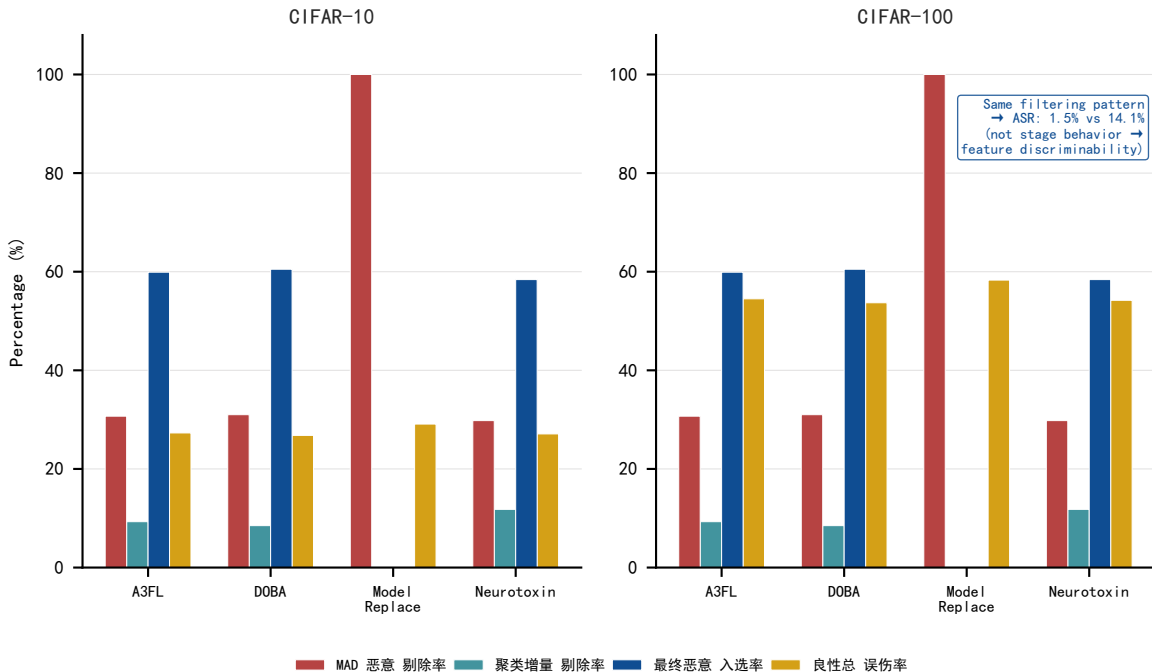
APRA Stage-Level Filtering Behavior — CIFAR-10 vs CIFAR-100
