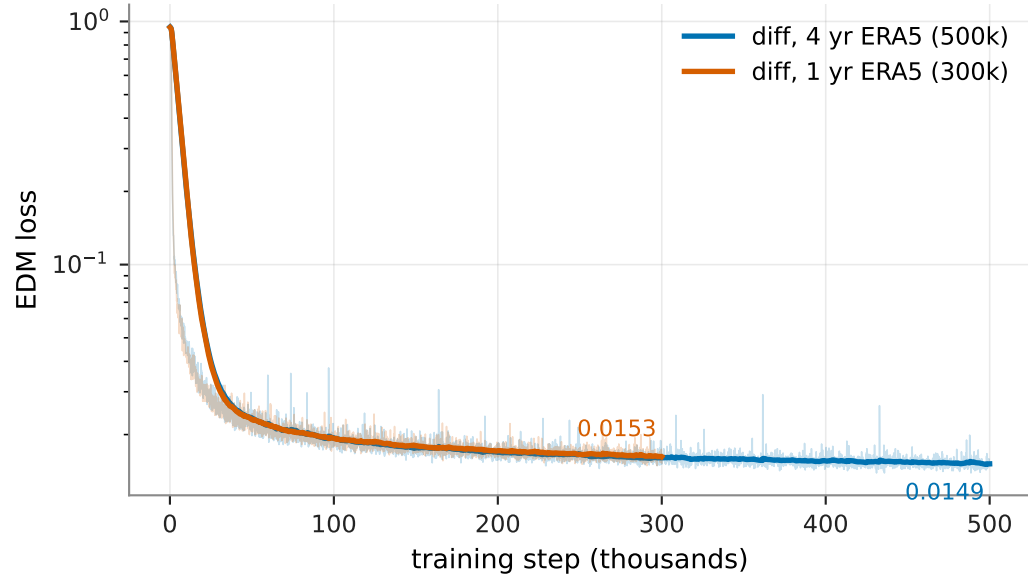
A. Training loss falls monotonically
