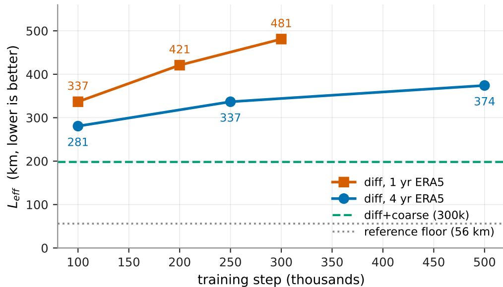
B. Effective resolution gets WORSE — in both runs
