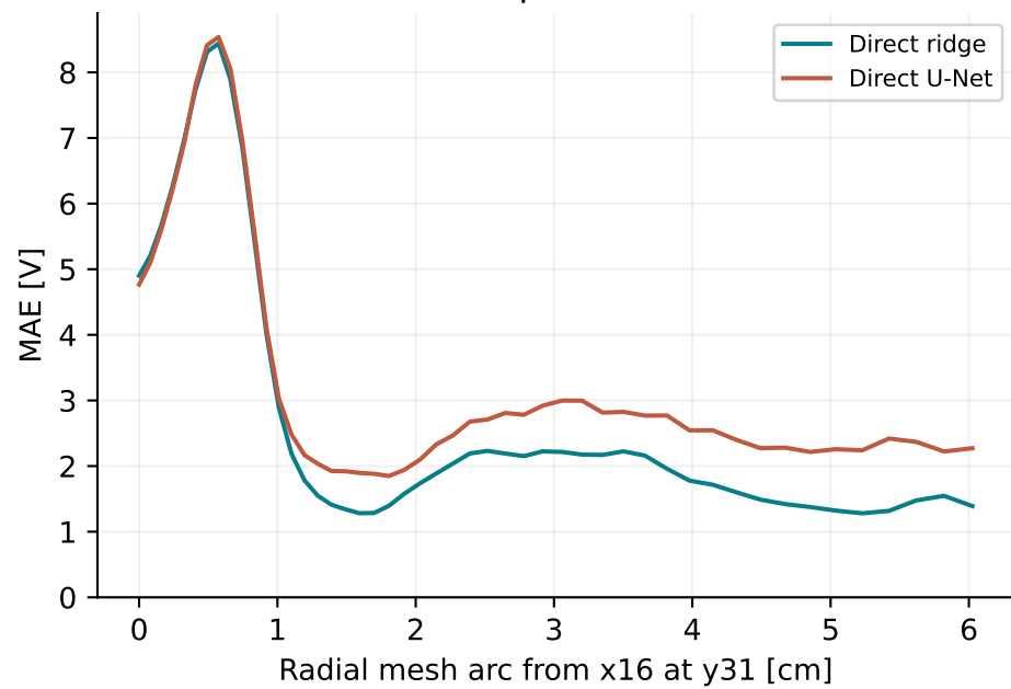
Native-cell prediction error
