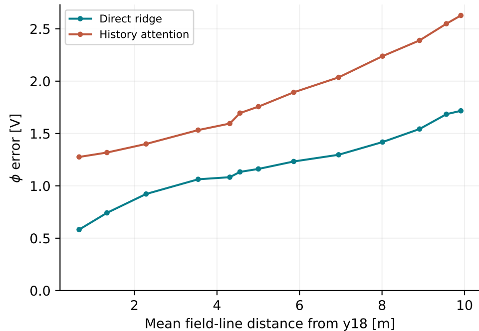
Full-field MAE
