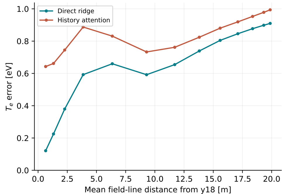
Full-field MAE
