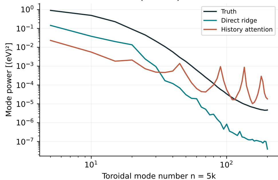
Toroidal power spectrum
