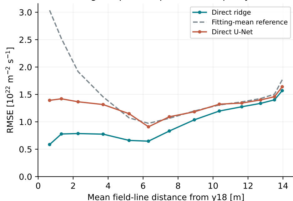
Signed parallel particle-flux proxy
