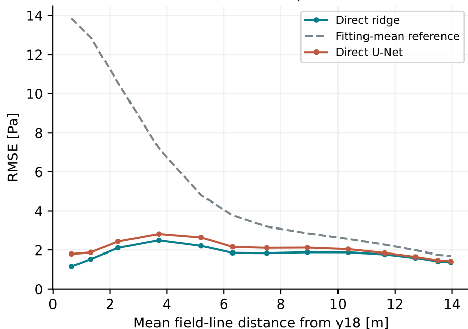
Derived electron pressure
