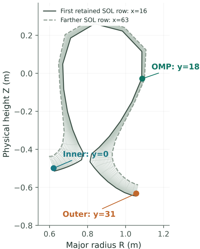
(b) A poloidal cut through that mesh
