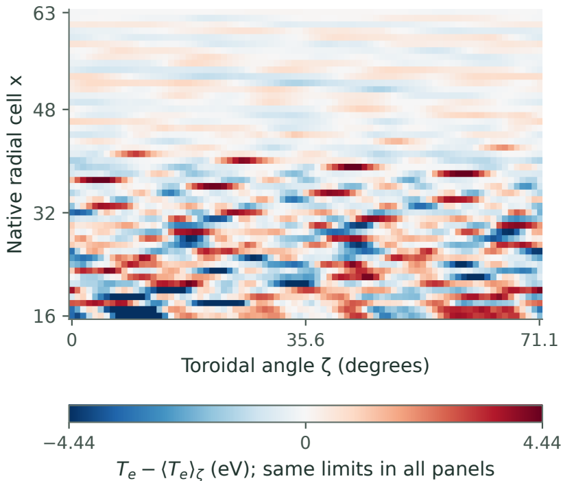
(b) Upstream pushed to outer 13.7000 ms · 54/3888 cells saturated
