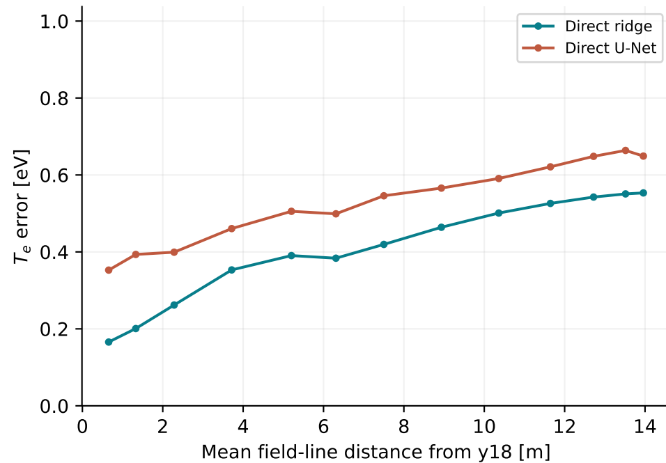
Full-field MAE
