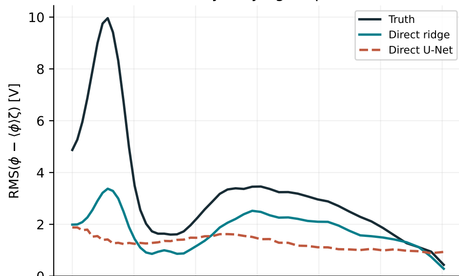
RMS - truth · magnified
