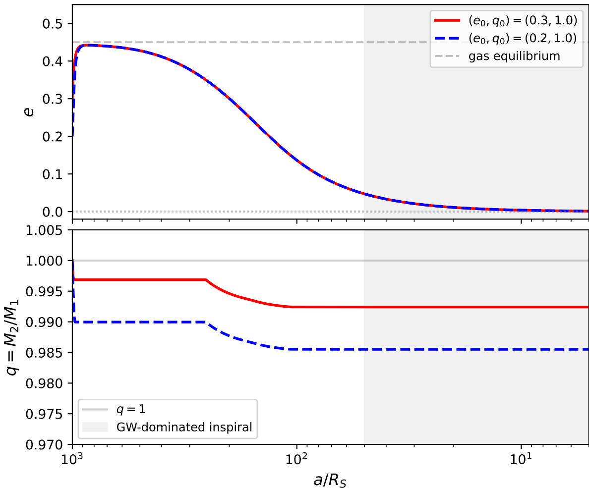
(e, q) evolution from a_0 = 10^3 R_S to 5R_S ( M = 10^7 M_\odot , \dot{M}_b = 100 \dot{M}_{\text{Edd}} )
