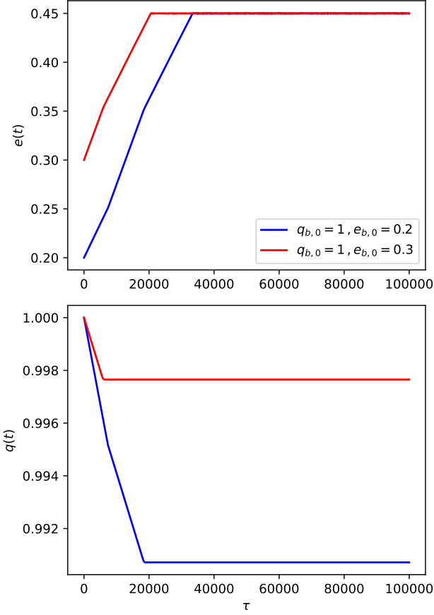
Figure 14. Evolution of binaries away from equal-mass. We depict the result of our numerical integration of equation 12 for e_{b,0}, q_{b,0} = (0.2, 1.0) (blue) and (0.3, 1.0) (red). The y-axes are e(t) (upper) and q(t) (lower) of the binary and the x-axes are time in units of each binary’s orbital period.
