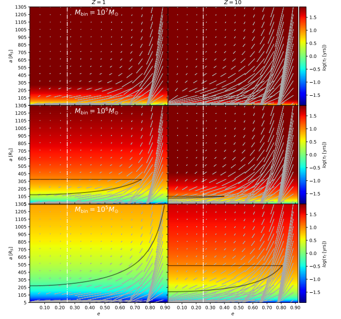
Figure 13. The region of parameter space that satisfies the above time constraints (within black lines) for various binary masses at various redshifts. The x-axis of each panel is the eccentricity e_b , the y-axis is the a_b in Schwarzschild radii, and \tau_f is reported in the observer frame. The gray lines represent the net effect of 10 orbits of GW radiation on the eccentricity and semi-major axis of each BBH.
