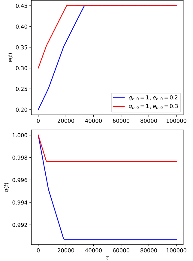
Figure 14. Evolution of binaries away from equal-mass. We depict the result of our numerical integration of equation 12 for e_{b0}, q_{b0} = (0.2, 1.0) (blue) and (0.3, 1.0) (red). The y-axes are e(t) (upper) and q(t) (lower) of the binary and the x-axes are time in units of each binary's orbital period.
