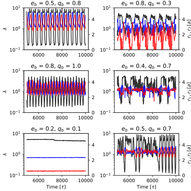
Figure 8. Comparison between the time-series of \lambda(t) (black), r_1(t) (blue), and r_2(t) (red). Clockwise from upper left we display e_b, q_b = (0.5, 0.8) , (0.8, 0.3) , (0.4, 0.7) , (0.5, 0.7) , (0.2, 0.1) , and 0.8, 1.0 . We find that the BHs position with respect to the cavity does not determine the components’ relative accretion rates.
