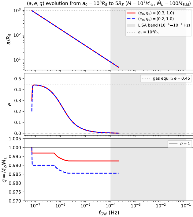
Figure 14. Extended integration of equation 12 from a_0 = 10^3 R_S down to a = 5 R_S for the (e_b, q_b) = (0.2, 1.0) (blue) and (0.3, 1.0) (red) cases, with M_{\text{tot}} = 10^7 M_\odot and \dot{M}_b = 100 \dot{M}_{\text{Edd}} . Top: semi-major axis vs GW frequency. Middle: eccentricity vs frequency, showing initial growth toward the gas-driven equilibrium e \approx 0.45 followed by GW circularization. Bottom: mass ratio vs frequency. The mass-ratio deviation from unity established during the gas-dominated phase is preserved through GW-dominated inspiral and persists into the LISA frequency band (gray, 10^{-4} to 10^{-1} Hz). The minor step in q(t) around f_{\text{GW}} \sim 2 \times 10^{-6} Hz reflects the discrete grid resolution of the \dot{q}_{\text{gas}} lookup table (rounded to \Delta q_b = 0.1 ); the qualitative result is unchanged.
