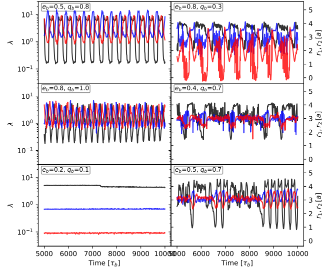
Figure 8. Comparison between the time-series of \lambda(t) (black, left log-axis), r_1(t) (blue), and r_2(t) (red) (right axis, in units of the binary semi-major axis a ). Time is in binary orbital periods \tau_b ; panels are plotted for 5000 \leq t/\tau_b \leq 10000 . Clockwise from upper-left: (e_b, q_b) = (0.5, 0.8) , (0.8, 0.3) , (0.4, 0.7) , (0.5, 0.7) , (0.2, 0.1) , and (0.8, 1.0) . We find that the BHs’ position with respect to the cavity does not determine the components’ relative accretion rates.
