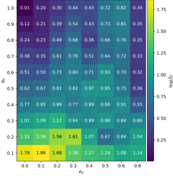
Figure 11. \tilde{\lambda} —The Eddington-normalized accretion-rate gauge \tilde{\lambda} \equiv (\max(\dot{M}_1, \dot{M}_2)) / (\min(\dot{M}_1, \dot{M}_2)) for our simulation suite, in \dot{M}_{\text{Edd}} units. The x-axis is the binary eccentricity e_b , and the y-axis is q_b , and the cell colors indicate \log \tilde{\lambda} . Combined with an assumed binary accretion rate \dot{M}_b , \tilde{\lambda} converts directly into the value Eddington-normalized accretion rate of \log(\tilde{\lambda}) each BH, allowing the jet-launching regime (single, dual, or flickering — see Fig. 10) to be predicted from (q_b, e_b) alone for a given \dot{M}_b .
