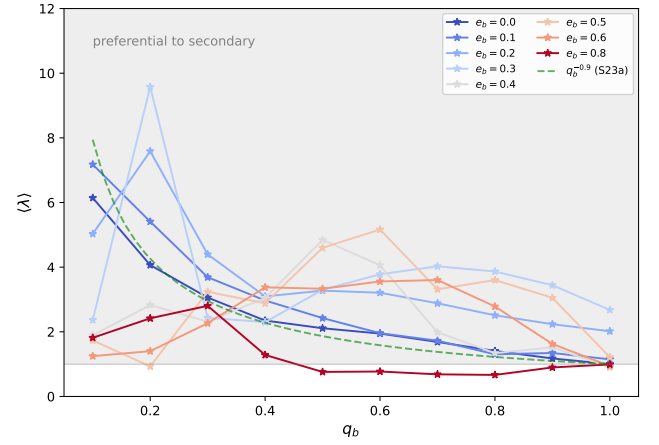
Figure 4. \langle\lambda\rangle across Time-averaged accretion-rate ratio \langle\lambda\rangle = \langle\dot{M}_2/\dot{M}_1\rangle as a function of q_b (x-axis) and e_b (line color). \langle\lambda\rangle is represented on the y-axis. The gray-shaded region marks \langle\lambda\rangle > 1 , q_b is on where the x-axis, and the color represents e_b simulation labelled “secondary” accretes preferentially. We also plot the power-law fitting to \langle\lambda\rangle of q_b^{-0.9} from in the The dashed green line is the q_b^{-0.9} power-law fit reported by Siwek et al. (2023a) for circular binaries.
