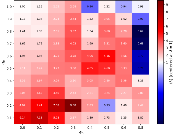
Figure 5. A heat-map displaying the time-averaged Heat-map of \lambda(t) - \langle \lambda \rangle across our simulation suite. The diverging colormap is centered at \lambda = 1 : red cells indicate preferential accretion onto the (apocenter-defined) secondary BH, blue cells indicate preferential accretion onto the primary. More eccentric, more unequal mass binaries seem to accrete more preferentially, though the trend is not monotonic.
