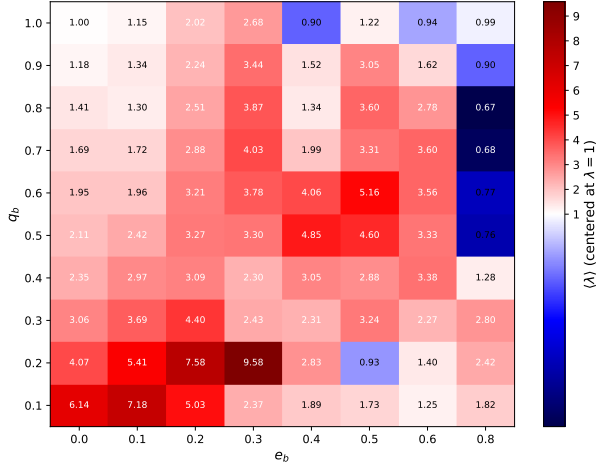
Figure 5. Heat-map of the time-averaged \langle \lambda \rangle = \langle \dot{M}_2 / \dot{M}_1 \rangle across the suite. The diverging colormap is centered at \lambda = 1 : red cells indicate preferential accretion onto the (apocenter-defined) secondary BH, blue cells indicate preferential accretion onto the primary. More eccentric, more unequal mass binaries tend to accrete more preferentially, though the trend is not monotonic.
