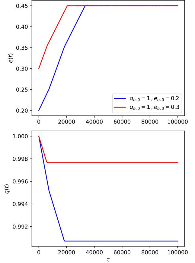
Figure 15. Evolution of binaries away from equal-mass. We depict the result of our numerical integration of equation 12 for e_{b,0}, q_{b,0} = (0.2, 1.0) (blue) and (0.3, 1.0) (red). The y-axes are e(t) (upper) and q(t) (lower) of the binary and the x-axes are time in units of each binary’s orbital period.
