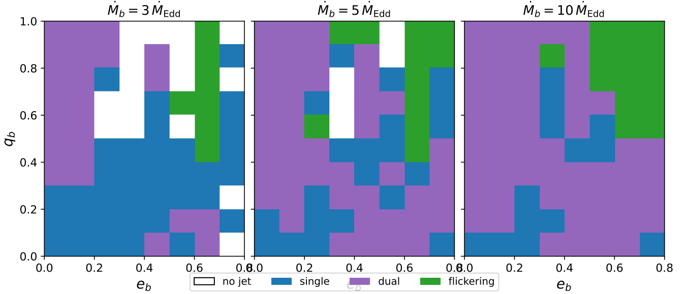
Figure 13. Jet-regime classification as a function of (e_b, q_b) for three values of the binary accretion rate \dot{M}_b \in \{3, 5, 10\} \dot{M}_{\text{Edd}} . Each cell is colored by the regime (white: no jet; blue: single; purple: dual; green: flickering) using the same threshold and duration criteria as Fig. 11 ( \dot{M}_i > 1.1 \dot{M}_{\text{Edd},i} sustained for \geq 50 \tau_b ). The three values bracket the range over which all three regimes coexist: at \dot{M}_b = 3 singles dominate with dual at the low- e_b , low- q_b edge and flickering along e_b \approx 0.6 ; at \dot{M}_b = 5 duals fill most of the grid and flickering migrates upward in q_b ; at \dot{M}_b = 10 duals dominate and flickering occupies the high- q_b , high- e_b corner.
