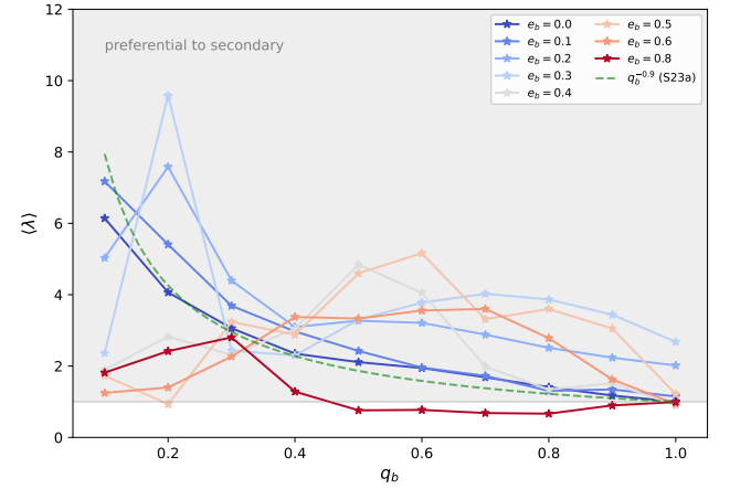
Figure 4. Time-averaged accretion-rate ratio \langle \lambda \rangle = \langle \dot{M}_2 / \dot{M}_1 \rangle as a function of q_b (x-axis) and e_b (line color). The gray-shaded region marks \langle \lambda \rangle > 1 , where the simulation labelled “secondary” accretes preferentially. The dashed green line is the q_b^{-0.9} power-law fit reported by Siwek et al. (2023a) for circular binaries.
