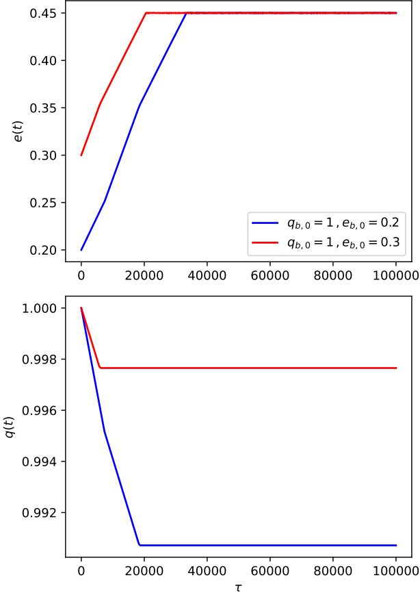
Figure 15. Evolution of binaries away from equal-mass. We depict the result of our numerical integration of equation 12 for e_{b,0}, q_{b,0} = (0.2, 1.0) (blue) and (0.3, 1.0) (red). The y-axes are e(t) (upper) and q(t) (lower) of the binary and the x-axes are time in units of each binary’s orbital period.
