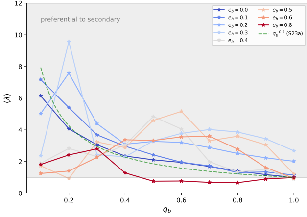
Figure 4. \langle \lambda \rangle across Time-averaged accretion-rate ratio \langle \lambda \rangle = \langle \dot{M}_2 / \dot{M}_1 \rangle as a function of q_b (x-axis) and e_b (line color). \langle \lambda \rangle is represented on the y-axis. The gray-shaded region marks \langle \lambda \rangle > 1 , q_b is on the x-axis, and the color represents e_b simulation labelled “secondary” accretes preferentially. We also plot the power-law fitting to \langle \lambda \rangle of q_b^{-0.9} from Siwek et al. (2023a) in the dashed green line is the q_b^{-0.9} power-law fit reported by Siwek et al. (2023a) for circular binaries.
