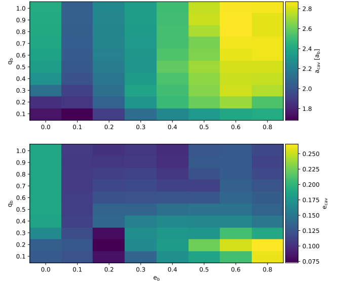
Figure 3. Reproduction of Figure 18 from DeLaurentiis & Rafikov (2025) displaying the semi-major axis and eccentricity of the cavities of our simulations with varying binary eccentricity and mass ratio. The cavity is characterized by the m = 1 Fourier mode of the CBD cavity
