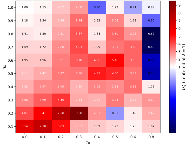
Figure 5. A heat-map displaying the time-averaged Heat-map of \lambda(t) across our simulation suite. The diverging colormap is centered at \lambda = 1 : red cells indicate preferential accretion onto the (apocenter-defined) secondary BH, blue cells indicate preferential accretion onto the primary. More eccentric, more unequal mass binaries seem tend to accrete more preferentially, though the trend is not monotonic.
