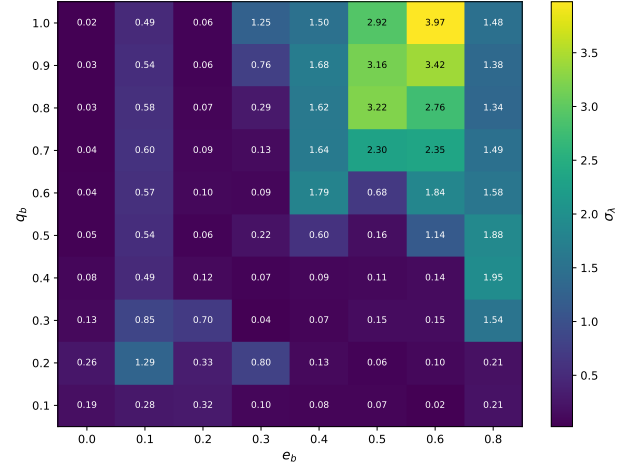
Figure 2. A heat-map displaying Heat-map of \sigma_\lambda , the standard deviation of \lambda(t) to indicate over the difference post-instability ( t > 3000\tau_b ) portion of the simulation. Larger values (brighter) indicate stronger time-variability of preferential accretion. The variability peaks broadly in oscillation-behavior across our simulations the high- e_b , intermediate- q_b region of parameter space.
