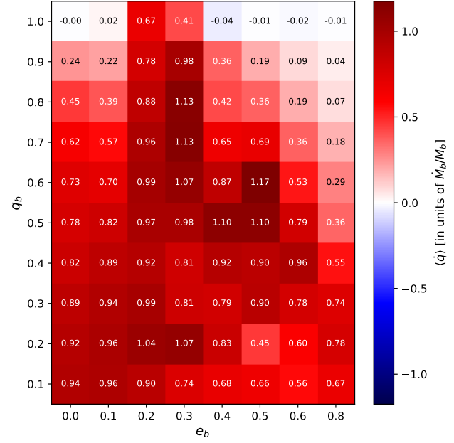
Figure 10. The average time-averaged rate of change of the binary mass-ratio, \langle \dot{q} \rangle , for our simulation suite, in M_b/M_b units. The x-axis is the binary eccentricity e_b and the y-axis is the binary mass-ratio q_b . The diverging colormap is centered at \langle \dot{q} \rangle = 0 : red cells indicate the value of binary evolves toward q = 1 (positive \langle \dot{q} \rangle ), blue cells away from q = 1 . Most q_b < 1 cells are positive (driven toward equal mass); the q_b = 1 row is represented as color mostly consistent with zero, with notable exceptions at e_b = 0.2 and 0.3 where the binary evolves away from unity (§3.2).
