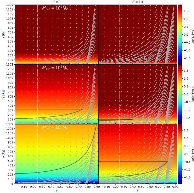
Figure 12. The region of parameter space that satisfies the above time constraints (within black lines) for various binary masses at various redshifts. The x-axis of each panel is the eccentricity e_b , the y-axis is the a_b in Schwarzschild radii, and \tau_f is reported in the observer frame. The gray lines represent the net effect of 10 orbits of GW radiation on the eccentricity and semi-major axis of each BBH.
