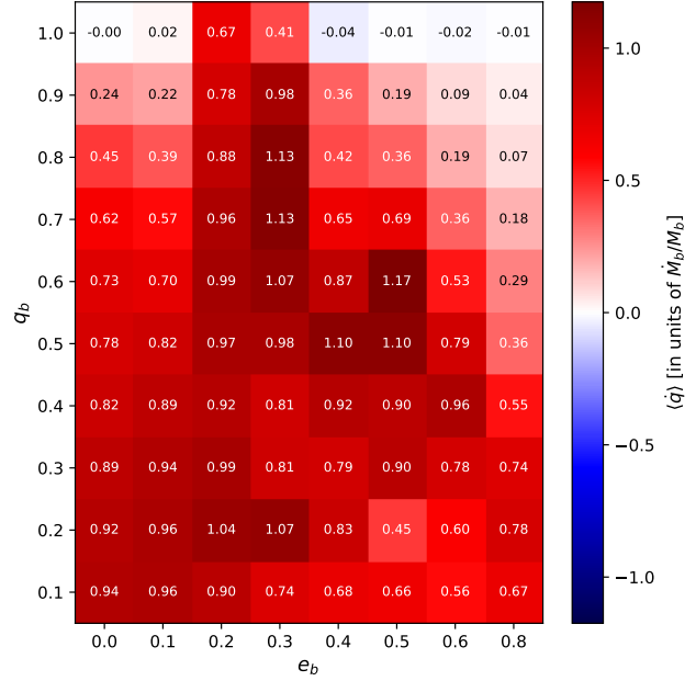
Figure 9. The average time-averaged rate of change of the binary mass ratio, \langle \dot{q} \rangle , for our the simulation suite, in \dot{M}_b/M_b units. The x-axis is the binary eccentricity e_b and the y-axis is the binary mass ratio q_b and. The diverging colormap is centered at \langle \dot{q} \rangle = 0 : red cells indicate the value of binary evolves toward q = 1 (positive \langle \dot{q} \rangle ), blue cells away from q = 1 . Most q_b < 1 cells are positive (driven toward equal mass); the q_b = 1 row is represented as color mostly consistent with zero, with notable exceptions at e_b = 0.2 and 0.3 where the binary evolves away from unity (§3.2).
