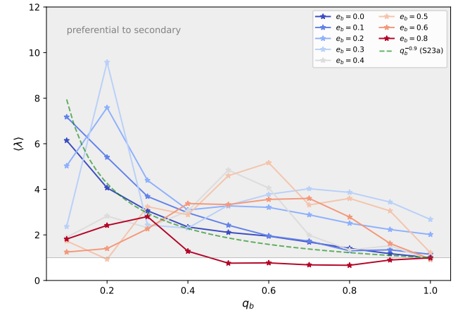
Figure 4. \langle \lambda \rangle across Time-averaged accretion-rate ratio \langle \lambda \rangle = \langle \dot{M}_2 / \dot{M}_1 \rangle as a function of q_b (x-axis) and e_b (line color). \langle \lambda \rangle is represented on the y-axis. The gray-shaded region marks \langle \lambda \rangle > 1 , q_b is on where the x-axis, and the color represents e_b simulation labelled “secondary” accretes preferentially. We also plot the power-law fitting to \langle \lambda \rangle of q_b^{-0.9} from in the The dashed green line is the q_b^{-0.9} power-law fit reported by Siwek et al. (2023a) for circular binaries.
