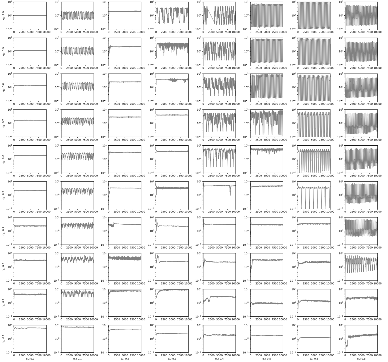
Figure 1. \lambda(t) —The accretion-rate ratio \lambda(t) \equiv \dot{M}_2(t)/\dot{M}_1(t) for our binary-simulation suite. Each panel represents a unique (e_b, q_b) simulation, with \lambda(t) on the y-axis and time on the x-axis (in units of binary orbital periods \tau_b ). The panel's position on the larger grid signifies its binary parameters, with e_b being constant along columns and increasing from left to right, and q_b being constant along rows and increasing from bottom to top.
