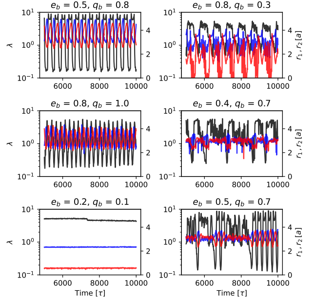
Figure 8. Comparison between the time-series of \lambda(t) (black), r_1(t) (blue), and r_2(t) (red). Clockwise from upper left we display e_b, q_b = (0.5, 0.8) , (0.8, 0.3) , (0.4, 0.7) , (0.5, 0.7) , (0.2, 0.1) , and 0.8, 1.0 . We find that the BHs position with respect to the cavity does not determine the components’ relative accretion rates.
