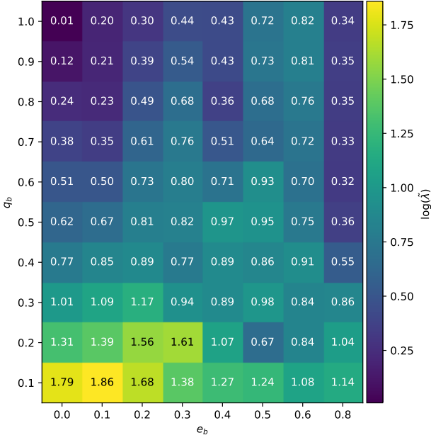
Figure 11. \tilde{\lambda} —The Eddington-normalized accretion-rate gauge \tilde{\lambda} \equiv \langle \max(\dot{M}_1, \dot{M}_2) \rangle / \langle \min(\dot{M}_1, \dot{M}_2) \rangle for our simulation suite, in \dot{M}_{\text{Edd}} units. The x-axis is the binary eccentricity e_b , and the y-axis is q_b , and the binary mass-ratio q_b ; cell colors indicate \log \tilde{\lambda} . Combined with an assumed binary accretion rate \dot{M}_b , \tilde{\lambda} converts directly into the value Eddington-normalized accretion rate of \log(\tilde{\lambda}) each BH, allowing the jet-launching regime (single, dual, or flickering — see Fig. 10) to be predicted from (q_b, e_b) alone for a given \dot{M}_b .
