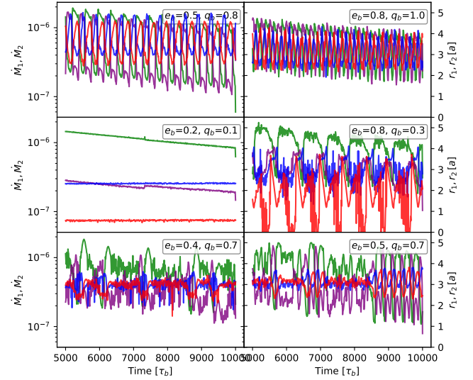
Figure 8. Six representative (e_b, q_b) simulations comparing the individual accretion rates \dot{M}_1 (purple, primary) and \dot{M}_2 (green, secondary), in units of the binary semi-major axis a , on the right axis. Time is in binary orbital periods \tau_b ; panels are plotted for 5000 \leq t/\tau_b \leq 10000 to focus on the post-transient regime. Reading row-by-row from the top, the panels show (e_b, q_b) = (0.5, 0.8), (0.8, 1.0), (0.2, 0.1), (0.8, 0.3), (0.4, 0.7), (0.5, 0.7) . The naive expectation that the BH closer to the cavity wall (smaller r ) should accrete more rapidly is satisfied only for (0.2, 0.1) (third panel); the other five panels show that proximity to the cavity wall does not directly determine which BH accretes preferentially.
