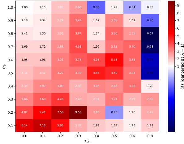
Figure 5. A heat-map displaying the time average Heat-map of \lambda(t) across our simulation suite. The diverging colormap is centered at \lambda = 1 : red cells indicate preferential accretion onto the (apocenter-defined) secondary BH, blue cells indicate preferential accretion onto the primary. More eccentric, more unequal mass binaries seem tend to accrete more preferentially, though the trend is not monotonic.
