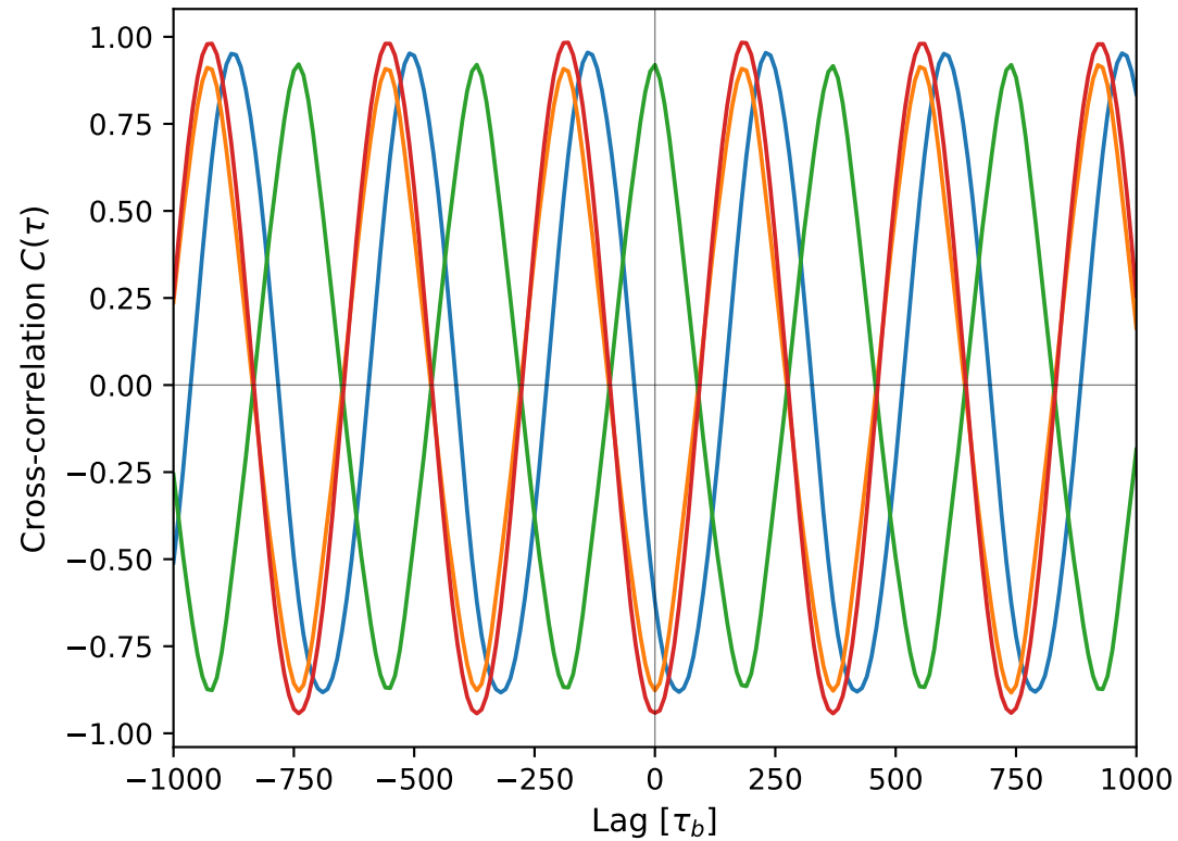
Clean period: (e_b, q_b) = (0.6, 1.0)
