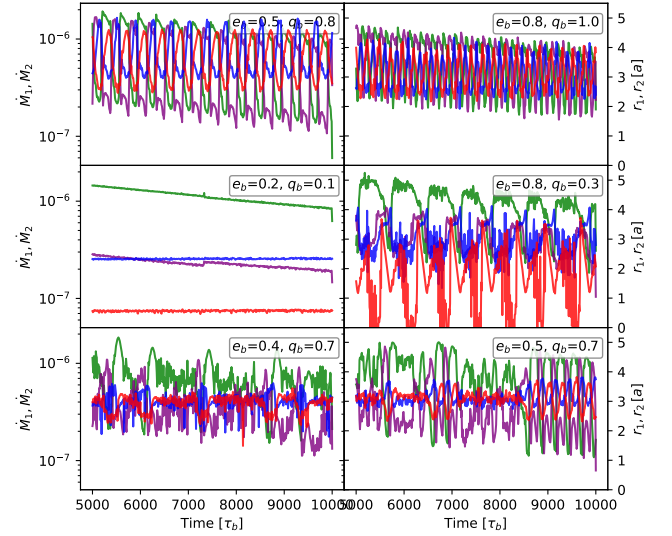
Figure 8. Six representative (e_b, q_b) simulations comparing the individual accretion rates \dot{M}_1 (purple, primary) and \dot{M}_2 (green, secondary), in units of the binary semi-major axis a , on the right axis. Time is in binary orbital periods \tau_b ; panels are plotted for 5000 \leq t/\tau_b \leq 10000 to focus on the post-transient regime. Reading row-by-row from the top, the panels show (e_b, q_b) = (0.5, 0.8), (0.8, 1.0), (0.2, 0.1), (0.8, 0.3), (0.4, 0.7), (0.5, 0.7) . The naive expectation that the BH closer to the cavity wall (smaller r ) should accrete more rapidly is satisfied only for (0.2, 0.1) (third panel); the other five panels show that proximity to the cavity wall does not directly determine which BH accretes preferentially.
