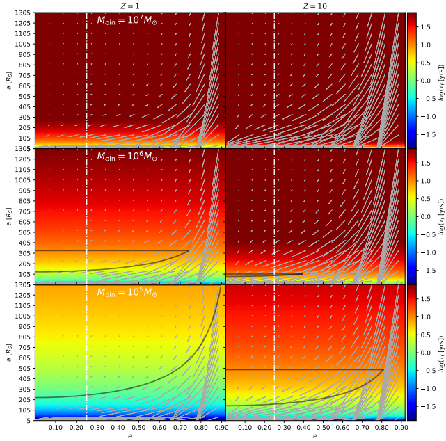
Figure 13. The region of parameter space that satisfies the above time constraints (within black lines) for various binary masses at various redshifts. The x-axis of each panel is the eccentricity e_b , the y-axis is the a_b in Schwarzschild radii, and \tau_f is reported in the observer frame. The gray lines represent the net effect of 10 orbits of GW radiation on the eccentricity and semi-major axis of each BBH.
