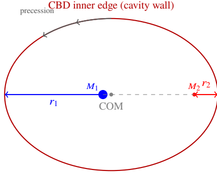
Figure 7. Schematic of the cavity geometry at apocenter for the locked-CBD case (here illustrated for an unequal-mass binary with q_b \ll 1 ). The CBD inner edge (red ellipse) is closer to the secondary on one side. The closest distances from each BH to the cavity wall are r_1 (primary, blue) and r_2 (secondary, red); in the locked configuration shown, r_1 > r_2 . As the disk precesses, the major axis of the ellipse rotates, and the orientations of r_1 and r_2 change accordingly.
