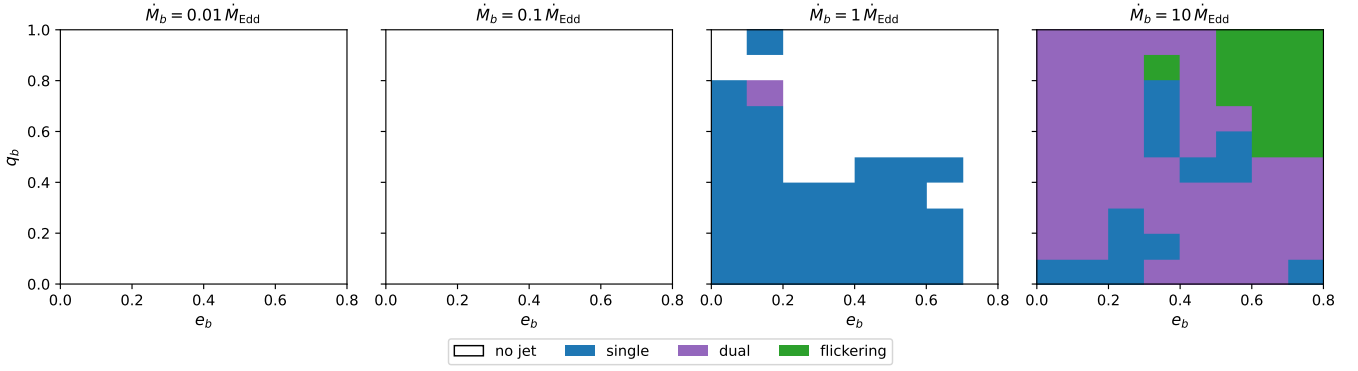
Figure 12. Jet-regime classification across (e_b, q_b) parameter space at four different assumed binary accretion rates: \dot{M}_b = 0.01, 0.1, 1, 10\dot{M}_{\text{Edd}} . Cells are color-coded by jet behavior: white = no jet, blue = single jet, purple = dual jet, green = flickering jet. The threshold and duration criteria are the same as in Fig. 10. The qualitative tapestry of regimes shifts dramatically with \dot{M}_b : at sub-Eddington rates almost no jets launch, at 1\dot{M}_{\text{Edd}} single-jet systems dominate the parameter space, and at super-Eddington rates dual and flickering jets fill the higher- q_b region. The flickering regime — our novel result — is broadest at \dot{M}_b = 10\dot{M}_{\text{Edd}} in the high- q_b , high- e_b corner.
