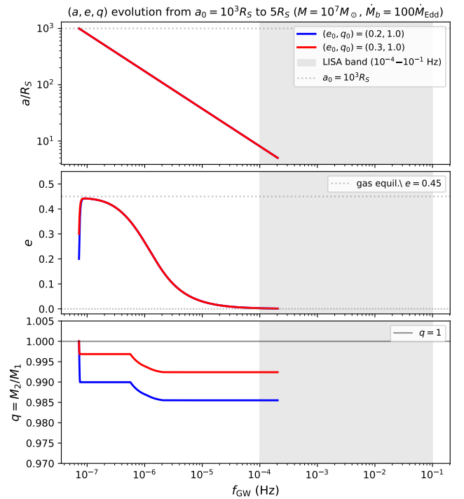
Figure 15. Extended integration of equation 12 from a_0 = 10^3 R_S down to a = 5 R_S for the (e_b, q_b) = (0.2, 1.0) (blue) and (0.3, 1.0) (red) cases, with M_{\text{tot}} = 10^7 M_\odot and \dot{M}_b = 100 \dot{M}_{\text{Edd}} . Top: semi-major axis vs GW frequency. Middle: eccentricity vs frequency, showing initial growth toward the gas-driven equilibrium e \approx 0.45 followed by GW circularization. Bottom: mass ratio vs frequency. The mass-ratio deviation from unity established during the gas-dominated phase is preserved through GW-dominated inspiral and persists into the LISA frequency band (gray, 10^{-4} to 10^{-1} Hz). The minor step in q(t) around f_{\text{GW}} \sim 2 \times 10^{-6} Hz reflects the discrete grid resolution of the \dot{q}_{\text{gas}} lookup table (rounded to \Delta q_b = 0.1 ); the qualitative result is unchanged.
