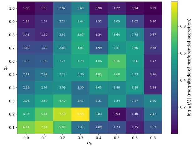
Figure 5. A heat-map displaying Heat-map showing the time-average magnitude of \lambda(t) - \langle \lambda \rangle preferential accretion across our simulation suite. More-eccentricThe colormap encodes |\log_{10} \langle \lambda \rangle| , more-unequal mass-binaries seem the deviation of the time-averaged accretion-rate ratio \langle \lambda \rangle = \langle \dot{M}_2 / \dot{M}_1 \rangle from unity (equal-rate accretion); brighter cells indicate stronger preferential accretion regardless of which BH happens to accrete more preferentially. In-cell labels show the actual \langle \lambda \rangle value: \langle \lambda \rangle > 1 in 71 of 80 cells (the secondary out-accretes the primary, though the trend standard preferential-accretion picture); \langle \lambda \rangle < 1 in the remaining 9 cells, of which most are q_b = 1 simulations where the apocenter labelling convention can be assigned either way (so \langle \lambda \rangle slightly above or below unity is not monotonic equally probable), plus a small number of unequal-mass dimspots (notably (e_b, q_b) = (0.5, 0.2) at \langle \lambda \rangle = 0.93 ) where the asymmetry is anomalous and discussed below.
