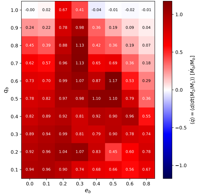
Figure 10. The average time-averaged rate of change of the binary mass ratio, \langle \dot{q} \rangle , for our simulation suite, in M_b/M_b units. The x-axis is the binary eccentricity e_b , and the y-axis is the binary mass ratio q_b . The diverging colormap is centered at \langle \dot{q} \rangle = 0 ; red cells indicate the value of binary evolves toward q = 1 (positive \langle \dot{q} \rangle ), blue cells away from q = 1 . Most q_b < 1 cells are positive (driven toward equal mass); the q_b = 1 row is represented as color mostly consistent with zero, with notable exceptions at e_b = 0.2 and 0.3 where the binary evolves away from unity (§3.2).
