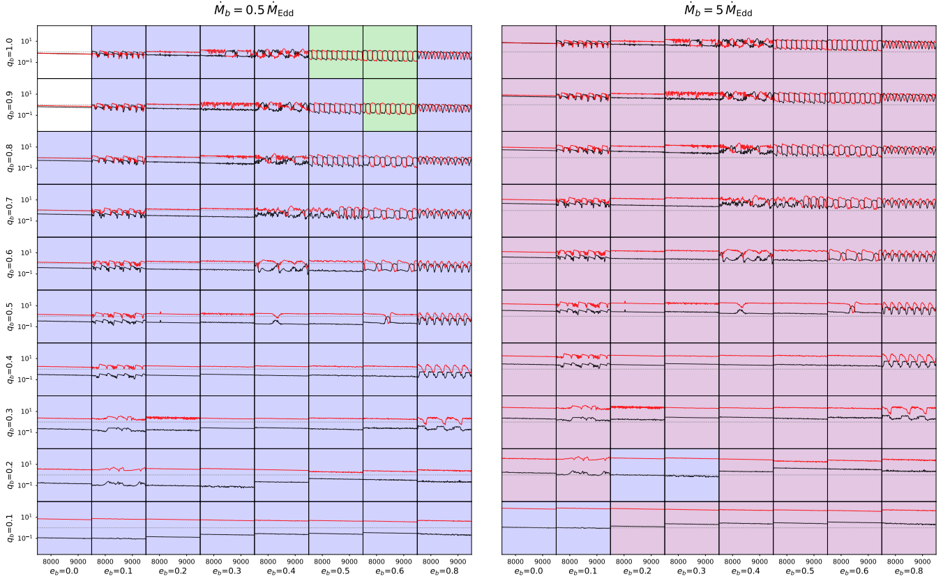
Figure 13. Reproduction of Fig. 11 at two bracketing values of the binary accretion rate: \dot{M}_b = 0.5 \dot{M}_{\text{Edd}} (left) and \dot{M}_b = 5 \dot{M}_{\text{Edd}} (right). Each cell shows the per-Eddington-normalized accretion rates of the primary (black) and secondary (red) on a log y-axis spanning [10^{-1}, 10^1] versus time in \tau_b within the post-transient window 7500 \leq t/\tau_b \leq 9500 ; the dashed gray horizontal marks the \dot{M}_i = \dot{M}_{\text{Edd},i} threshold. Backgrounds are colored by jet-regime classification using the same criteria as Fig. 11: white (no jet), blue (single), purple (dual), green (flickering). The figure makes explicit how the jet-regime tapestry shifts continuously with \dot{M}_b between the two extremes.
