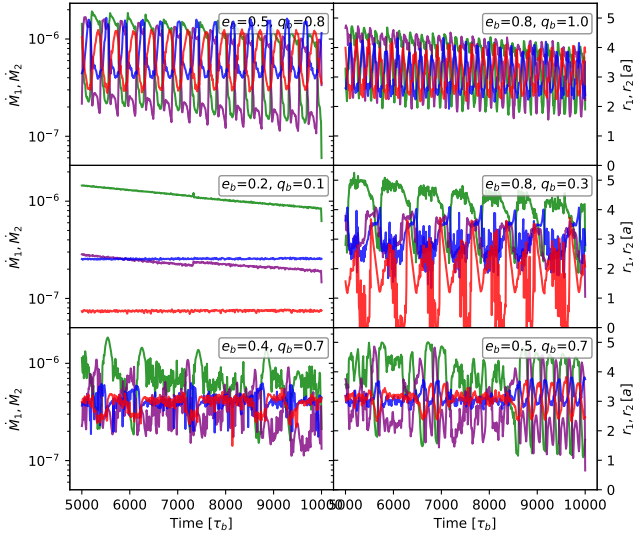
Figure 8. Comparison between Six representative (e_b, q_b) simulations comparing the time-series of \lambda(t) individual accretion rates \dot{M}_1 (blackpurple, primary) and \dot{M}_2 (green, r_1(t) -secondary) on the left log-axis to the BH-to-cavity-edge distances r_1 (blue, primary) and r_2(t) (red, secondary), in units of the binary semi-major axis a , on the right axis. Clockwise Time is in binary orbital periods \tau_b ; panels are plotted for 5000 \leq t/\tau_b \leq 10000 to focus on the post-transient regime. Reading row-by-row from upper-left we display e_b, q_b = (0.5, 0.8) , (0.8, 1.0) , (0.8, 0.3) , (0.5, 0.7) , (0.2, 0.1) , (0.4, 0.7) , and (0.5, 0.7) . We find The naive expectation that the BHs position with respect BH closer to the cavity wall (smaller r ) should accrete more rapidly is satisfied only for (0.2, 0.1) (third panel); the other five panels show that proximity to the cavity wall does not directly determine the components' relative accretion rates which BH accretes preferentially.
