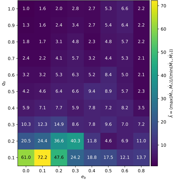
Figure 12. The Eddington-normalized accretion-rate gauge \tilde{\lambda} \equiv \langle \max(\dot{M}_1, \dot{M}_2) \rangle / \langle \min(\dot{M}_1, \dot{M}_2) \rangle for our simulation suite, in \dot{M}_{\text{Edd}} units. The x-axis is the binary eccentricity e_b and the y-axis is the binary mass-ratio q_b ; cell colors and labels indicate \tilde{\lambda} on a linear scale. Combined with an assumed binary accretion rate \dot{M}_b , \tilde{\lambda} converts directly into the Eddington-normalized accretion rate of each BH, allowing the jet-launching regime (single, dual, or flickering — see Fig. 11) to be predicted from (e_b, q_b) alone for a given \dot{M}_b .
