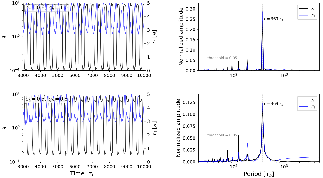
Figure 8. Time-series and power spectra for (e_b, q_b) = (0.6, 1.0) (top row) and (0.5, 0.8) (bottom row), illustrating the period match between \lambda(t) and the cavity-orientation proxy r_1(t) . Left column: \lambda(t) (black, left log-axis) and r_1(t) (blue, right axis in units of a ) over the post-transient window 3000 \leq t/\tau_b \leq 10000 ( N = 701 samples at the snapshot cadence of 10\tau_b ). Right column: normalized rFFT amplitudes |\tilde{X}(f)|/\sum_f |\tilde{X}(f)| as a function of period \tau = 1/f ; the dotted line marks the 0.05 amplitude threshold used in Fig. 6. Both signals peak cleanly at \tau \approx 369\tau_b in each simulation, demonstrating that \lambda(t) variability tracks the precessing cavity.
