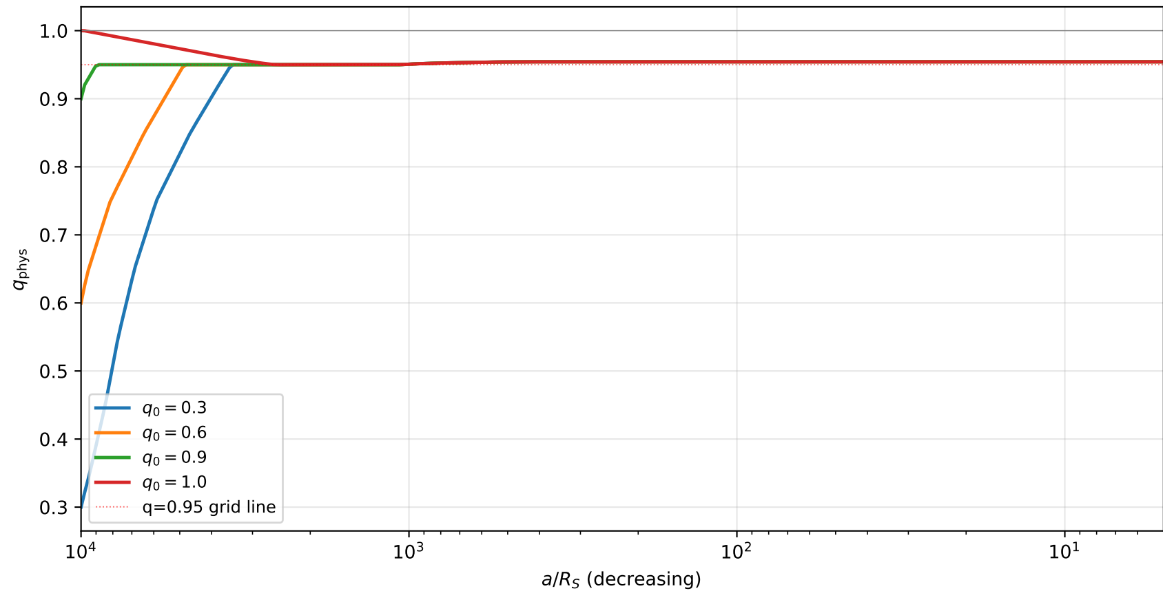
T3: q-evolution from different q_0 , e_0 = 0.2 , \dot{M}_b = 100 Edd, current lookup
