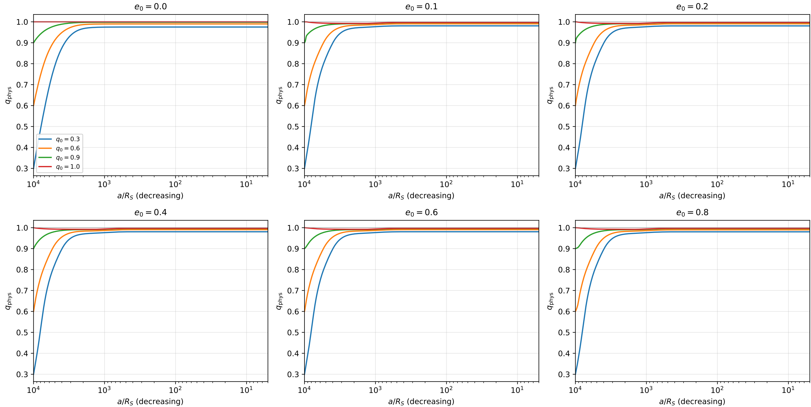
T3 (bilinear): q-evolution from different q_0 , fixed \dot{M}_{\text{bin}}=100 \text{ Edd}
