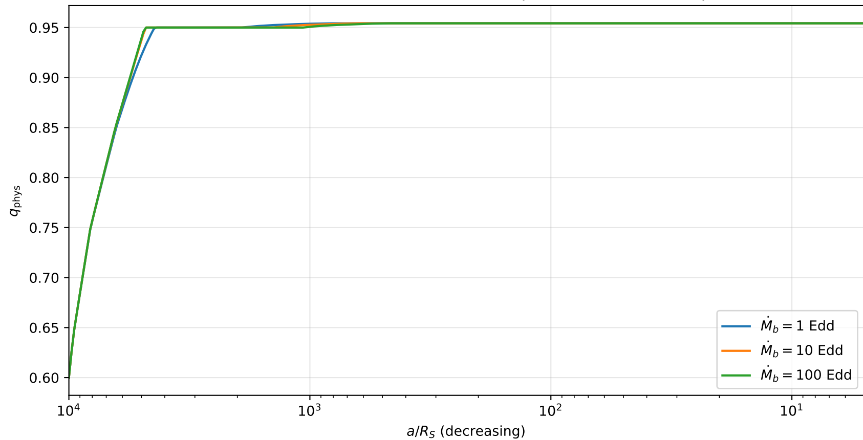
T4: \dot{M}_b invariance check — e_0 = 0.2, q_0 = 0.6 , current lookup
