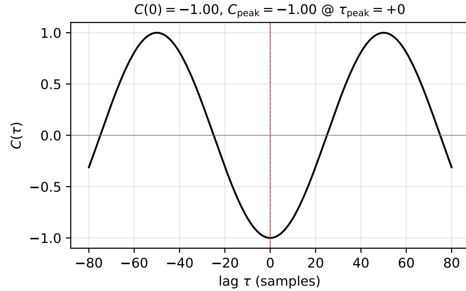
Toy model: phase-shift signatures in C(\tau) between \lambda(t) proxy and r_l(t) proxy. Period T = 100 .
