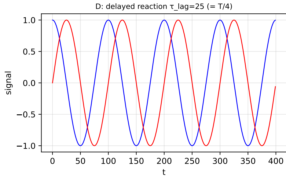
Toy model: phase-shift signatures in C(\tau) between \lambda(t) proxy and r_l(t) proxy. Period T = 100 .
