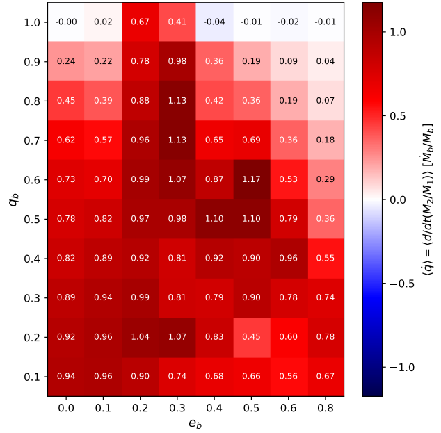
Figure 10. The average time-averaged rate of change of the binary mass ratio, \langle \dot{q} \rangle , for our simulation suite, in \dot{M}_b/M_b units. The x-axis is the binary eccentricity e_b , and the y-axis is the binary mass ratio q_b . The diverging colormap is centered at \langle \dot{q} \rangle = 0 : red cells indicate the value of binary evolves toward q = 1 (positive \langle \dot{q} \rangle ), blue cells away from q = 1 . Most q_b < 1 cells are positive (driven toward equal mass); the q_b = 1 row is represented as color mostly consistent with zero, with notable exceptions at e_b = 0.2 and 0.3 where the binary evolves away from unity (§3.2).
