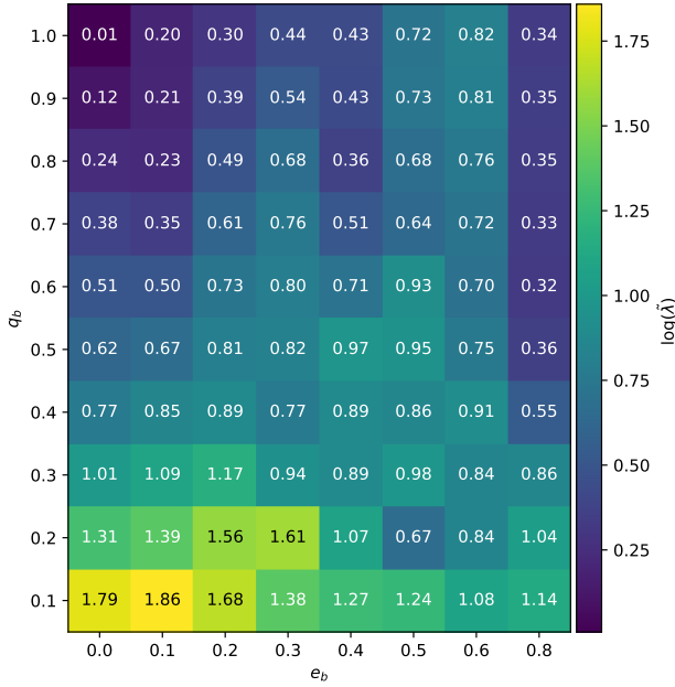
Figure 12. \tilde{\lambda} —The Eddington-normalized accretion-rate gauge \tilde{\lambda} \equiv \langle \max(\dot{M}_1, \dot{M}_2) \rangle / \langle \min(\dot{M}_1, \dot{M}_2) \rangle for our simulation suite, in \dot{M}_{\text{Edd}} units. The x-axis is the binary eccentricity e_b , and the y-axis is q_b , and the binary mass-ratio q_b ; cell colors indicate \log \tilde{\lambda} . Combined with an assumed binary accretion rate \dot{M}_b , \tilde{\lambda} converts directly into the value Eddington-normalized accretion rate of \log(\tilde{\lambda}) each BH, allowing the jet-launching regime (single, dual, or flickering — see Fig. 11) to be predicted from (e_b, q_b) alone for a given \dot{M}_b .
