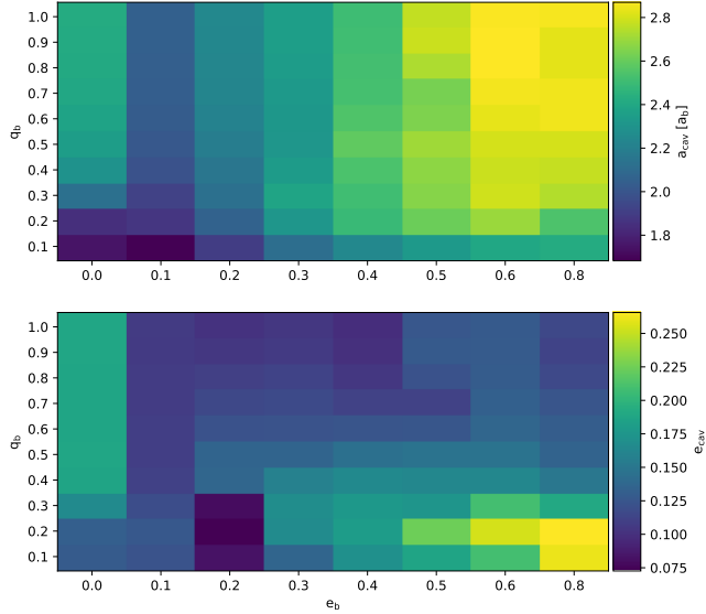
Figure 3. Reproduction of Figure 18 from DeLaurentiis & Rafikov (in preparation), displaying the semi-major axis and eccentricity of the cavities of our simulations with varying binary eccentricity and mass ratio. The cavity is characterized by the m = 1 Fourier mode of the CBD cavity
