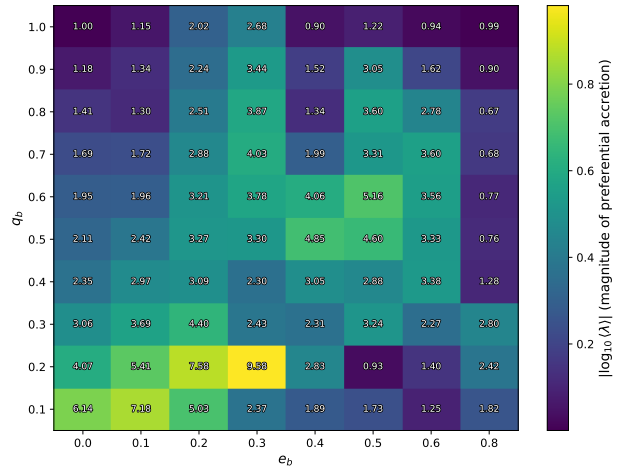
Figure 5. A heat-map displaying Heat-map showing the time-average magnitude of \lambda(t) - \langle \lambda \rangle preferential accretion across our simulation suite. The colormap encodes |\log_{10} \langle \lambda \rangle| , more unequal mass binaries seem the deviation of the time-averaged accretion-rate ratio \langle \lambda \rangle = \langle \dot{M}_2 / \dot{M}_1 \rangle from unity (equal-rate accretion); brighter cells indicate stronger preferential accretion regardless of which BH happens to accrete more preferentially. In-cell labels show the actual \langle \lambda \rangle value: \langle \lambda \rangle > 1 in 71 of 80 cells (the secondary out-accretes the primary, though the trend standard preferential-accretion picture); \langle \lambda \rangle < 1 in the remaining 9 cells, of which most are q_b = 1 simulations where the apocenter labelling convention can be assigned either way (so \langle \lambda \rangle slightly above or below unity is not monotonically equally probable), plus a small number of unequal-mass dimspots (notably (e_b, q_b) = (0.5, 0.2) at \langle \lambda \rangle = 0.93 ) where the asymmetry is anomalous and discussed below.
