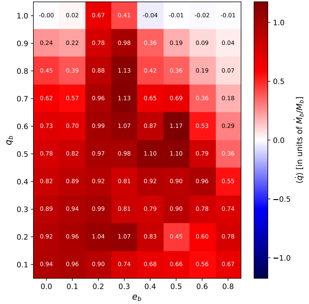
Figure 9. The average-time-averaged rate of change of the binary mass-ratio, \langle \dot{q} \rangle , for our simulation suite, in \dot{M}_b/M_b units. The x-axis is the binary eccentricity e_b and the y-axis is the binary mass-ratio q_b . The diverging colormap is centered at \langle \dot{q} \rangle = 0 : red cells indicate the value of binary evolves toward q = 1 (positive \langle \dot{q} \rangle ), blue cells away from q = 1 . Most q_b < 1 cells are positive (driven toward equal mass); the q_b = 1 row is represented as color mostly consistent with zero, with notable exceptions at e_b = 0.2 and 0.3 where the binary evolves away from unity (§3.2).
