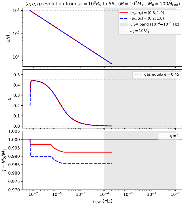
Figure 14. Extended integration of equation 12 from a_0 = 10^3 R_S down to a = 5 R_S for the (e_b, q_b) = (0.2, 1.0) (blue) and (0.3, 1.0) (red) cases, with M_{\text{tot}} = 10^7 M_\odot and M_b = 100 M_{\text{Edd}} . Top: semi-major axis vs GW frequency. Middle: eccentricity vs frequency, showing initial growth toward the gas-driven equilibrium e \approx 0.45 followed by GW circularization. Bottom: mass ratio vs frequency. The mass-ratio deviation from unity established during the gas-dominated phase is preserved through GW-dominated inspiral and persists into the LISA frequency band (gray, 10^{-4} to 10^{-1} Hz). The minor step in q(t) around f_{\text{GW}} \sim 2 \times 10^{-6} Hz reflects the discrete grid resolution of the \dot{q}_{\text{gas}} lookup table (rounded to \Delta q_b = 0.1 ); the qualitative result is unchanged.
