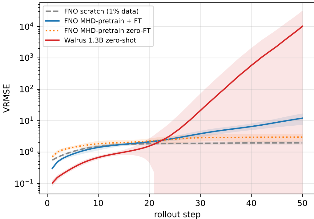
VRMSE vs rollout step (10 trajectories, shared window)
