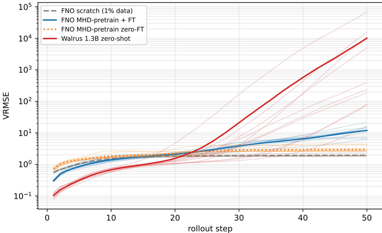
Per-trajectory rollout VRMSE (all four models overlaid)
