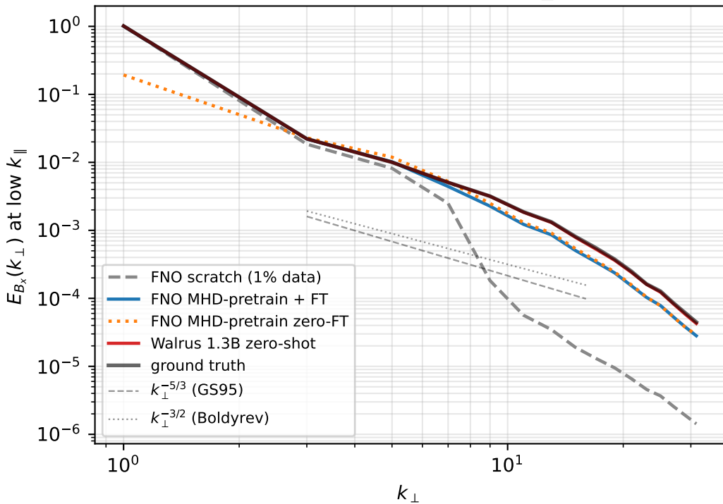
Perpendicular cascade at step 1 (B x channel)
